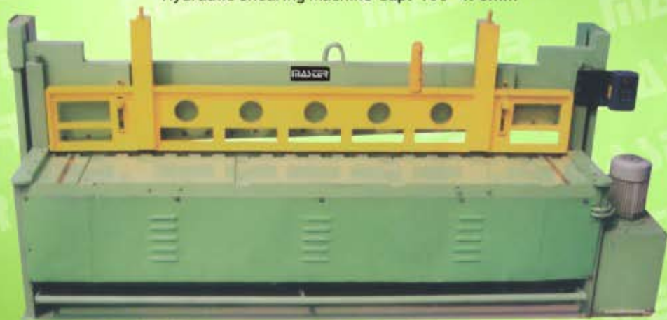
Hydraulic Shearing Machine Cap: 100" x 6mm
